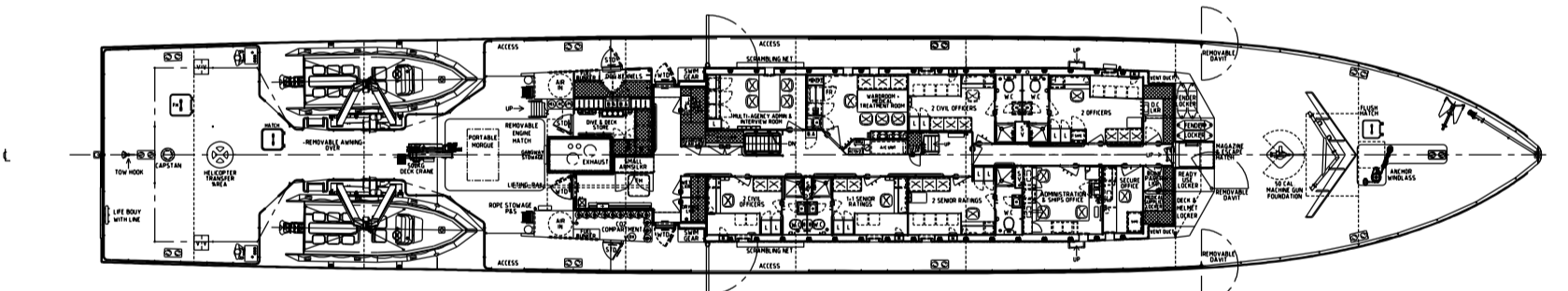
1 DECK
